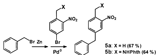
Scheme 3. First experiments in coupling of simple molecules to yield unsymmetrical diphenylmethanes for use in adrenaline receptor synthesis.
