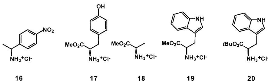
Scheme 7. More guest molecules 16–20 for binding experiments with 2a . All these molecules carry an additional alkyl or aryl substituent \alpha to the N atom and are rejected by the macrocyclic host molecule. Note that even the smallest amino acid derivative L-alanine methyl ester ( 18 ) does not bind to 2a .
