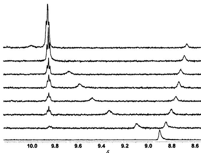
Figure 9. Drifting catechol OH signals during complex formation between pyridine-containing host 2b and noradrenaline in DMSO ( \delta = 9.85 : amide NH of host 8 , increasing during titration). The relative ratios of equivalents of 2b to noradrenaline from bottom to top are: 0, 0.25, 0.50, 0.75, 1.00, 1.25, 2.00, 4.75.
