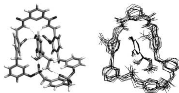
Figure 11. Left: Optimized complex geometry according to Monte Carlo simulations in water for the inclusion of noradrenaline inside the cavity of macrocyclic host 2b . Note the perfect preorganization by the pyridinecarboxamide head group, but also the kinked geometry in the diphenylmethane moiety. Right: Superimposed snapshots of the subsequent molecular dynamics calculation. Note the higher conformational flexibility of this complex compared with the corresponding assembly of noradrenaline with 2a .
