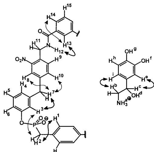
Figure 6. Proton assignments for intramolecular NOE measurements. Left: macrocycle 2a ; right: noradrenaline. Bold arrows: strong NOEs; thin arrows: medium NOEs.
