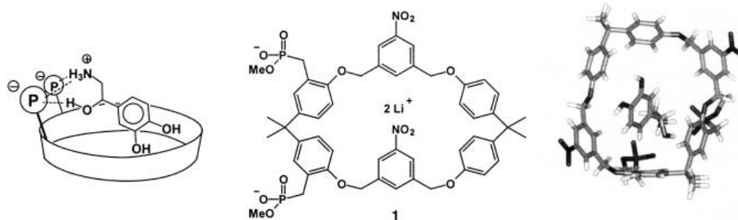
Figure 1. Macrocyclic host 1 with a hydrophobic cavity and peripheral phosphonates for ditopic recognition of adrenaline derivatives; left: schematic design; center: Lewis structure; right: conformational minimum calculated with Cerius 2 molecular simulations, force field: Dreiding 2.21.
