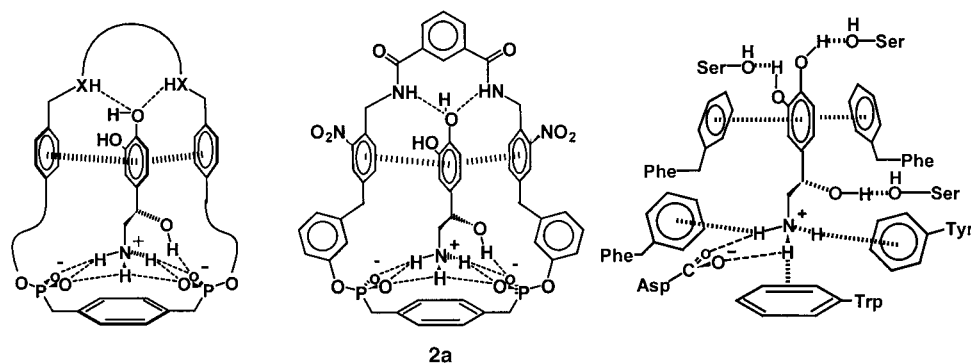
Scheme 1. Multipoint binding of adrenaline derivatives by biomimetic adrenaline host 2a with integral phosphonates. Left: schematic illustration of the planned interactions; middle: proposed binding mode; right: natural binding pattern of noradrenaline in the \beta -adrenergic receptor.
