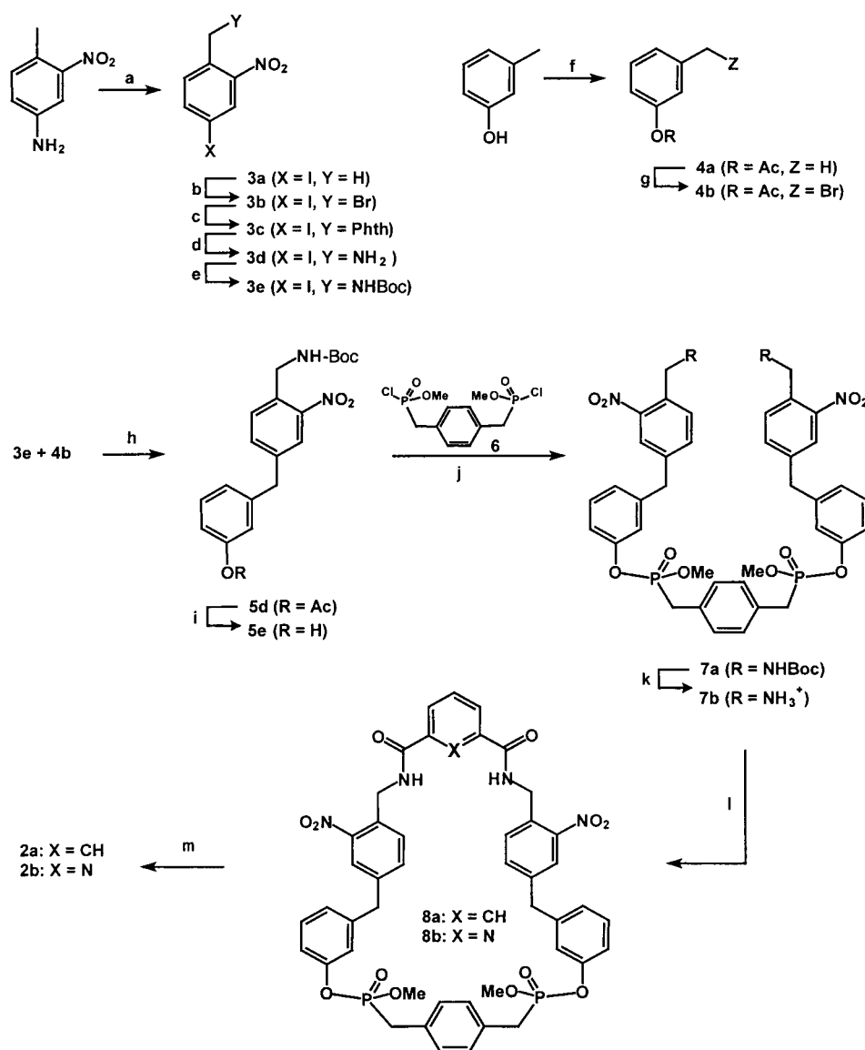
Scheme 5. Modular and convergent synthesis of hosts 2a and 2b from 4-amino-2-nitrotoluene, m -cresol, and p -xylylene bisphosphonic acid dimethyl ester dichloride; a) 1. NaNO 2 , 2. KI (61 %); b) NBS, CCl 4 (46 %); c) K phthalimide, [18]crown-6, toluene (94 %); d) N 2 H 4 , ethanol (65 %); e) Boc 2 O, CH 2 Cl 2 (95 %); f) Ac 2 O (89 %); g) NBS, CCl 4 (47 %); h) 1. Zn, reflux, 2. [Pd(PPh 3 ) 4 ]/DIBAL-H (58 %); i) K 2 CO 3 , methanol, RT (94 %); j) CH 2 Cl 2 , Et 3 N (57 %); k) TFA, CH 2 Cl 2 , 0 °C (99 %); l) isophthaloyl chloride or pyridine-2,6-dicarboxylic acid dichloride, Et 3 N, THF, benzene, RT ( 8a : 38 %; 8b : 32 %); m) LiBr, acetonitrile, 80 °C ( 2a : 66 %; 2b : 82 %).
