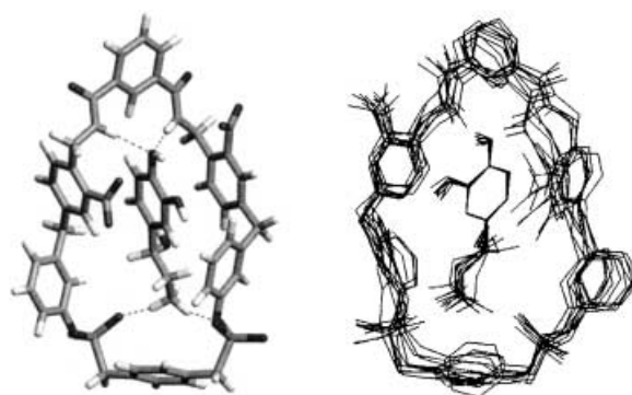
Figure 2. Left: Optimized complex geometry according to Monte Carlo simulations in water for the inclusion of noradrenaline inside the cavity of macrocyclic host 2a . Right: Superimposed snapshots of the subsequent molecular dynamics calculation.
