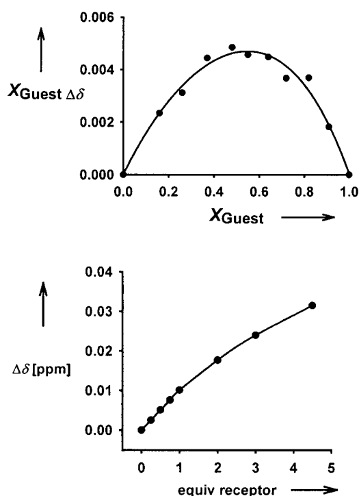
Figure 10. Top: Job plot for complex formation between host 2b and noradrenaline hydrochloride (CHN proton) in \text{D}_2\text{O} /methanol (1:1); bottom: NMR titration curve showing the complexation-induced shifts (CIS, CHN proton) for complex formation between host 2b and noradrenaline hydrochloride in the same solvent.
