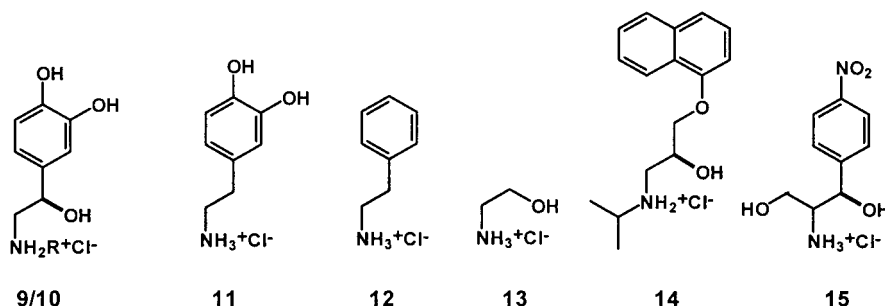
Scheme 6. Guest molecules 9–15 for binding experiments with 2a . The structure of adrenaline has been systematically truncated to establish the contribution of specific noncovalent interactions.
