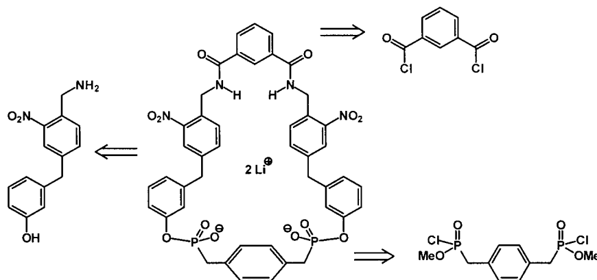
Scheme 2. Retrosynthetic analysis of macrocyclic host 2a : three building blocks open the path to a flexible modular synthesis with many variations.
