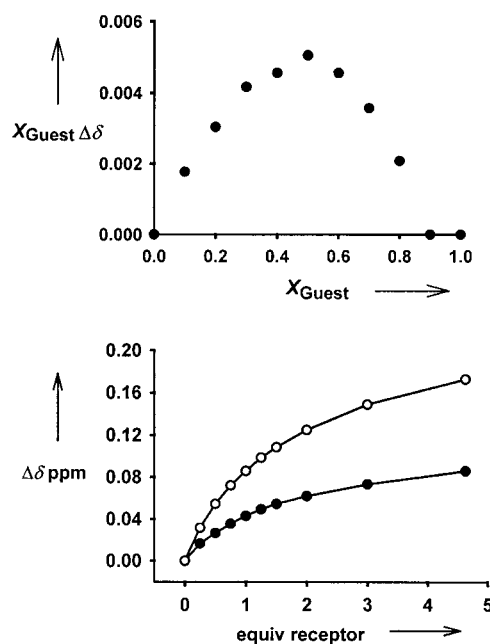
Figure 4. Top: Job plot for complex formation between host 2a and noradrenaline hydrochloride (CHN proton) in D_2O /methanol (1:1); bottom: NMR titration curve showing the complexation-induced shifts (CHN and CHO protons) for complex formation between host 2 and noradrenaline hydrochloride in methanol.
