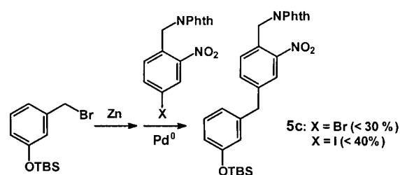
Scheme 4. More simple molecule couplings yielding unsymmetrical diphenylmethanes.
