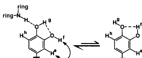
Figure 8. Shift in the catechol hydrogen bond equilibrium by complexation with host 2a and 2b ; experimental evidence from chemically induced shifts (CIS) and NOE measurements.
