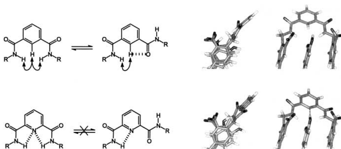
Figure 3. Top: Repulsive NH-CH interactions in isophthalamides; two views of the twisted head group in 2a . Bottom: Preorganization in pyridine-2,6-carboxamides; flat head group in 2b .
