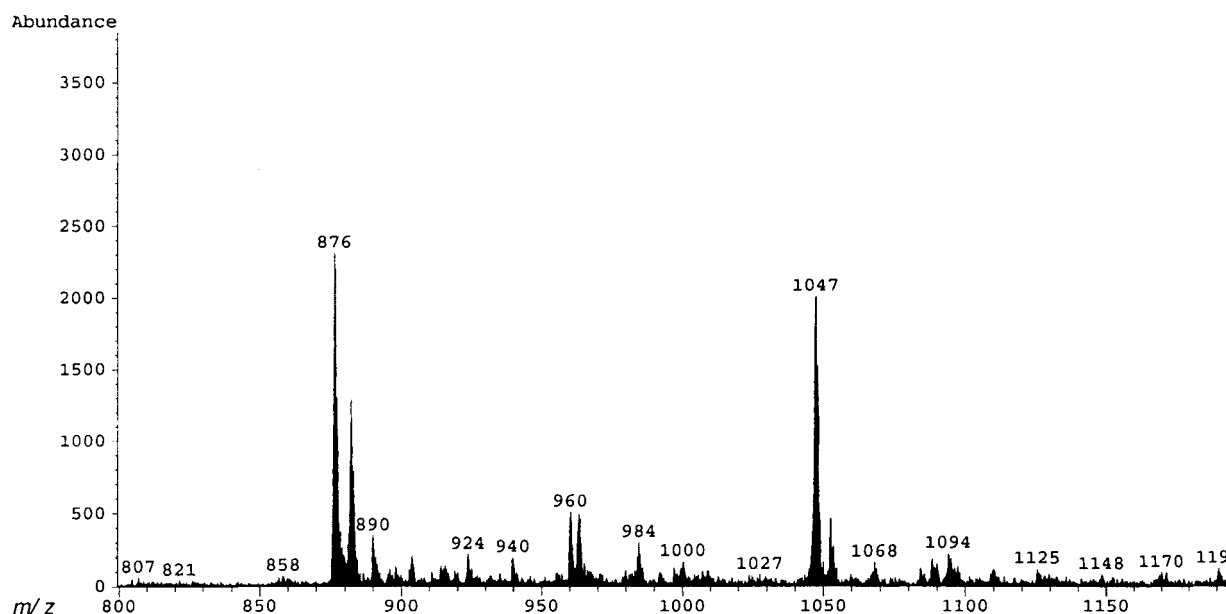
Figure 5. ESI-MS for the 1:1 complex of 2a with noradrenaline hydrochloride (mass range m/z 800–1200). Samples (20 \mu\text{L} ) were introduced as 10^{-7}\text{ M} solutions in methanol at flow rates of 20\text{ }\mu\text{L min}^{-1} . The major peaks are: m/z 876: 2a − , 873: 2a 2− + Li + , 890: 2a 3− + 2Li + , 1047: 2a 2− + noradrenaline + , 1054: 2a 3− + noradrenaline + + Li + .
