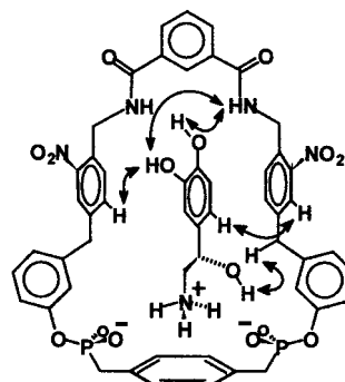
Figure 7. Intermolecular NOEs in the complex between host 2a and noradrenaline. The carbon-bound hydrogen atoms have been omitted for clarity. Bold characters show IR-sensitive functional groups involved in hydrogen bonds.
